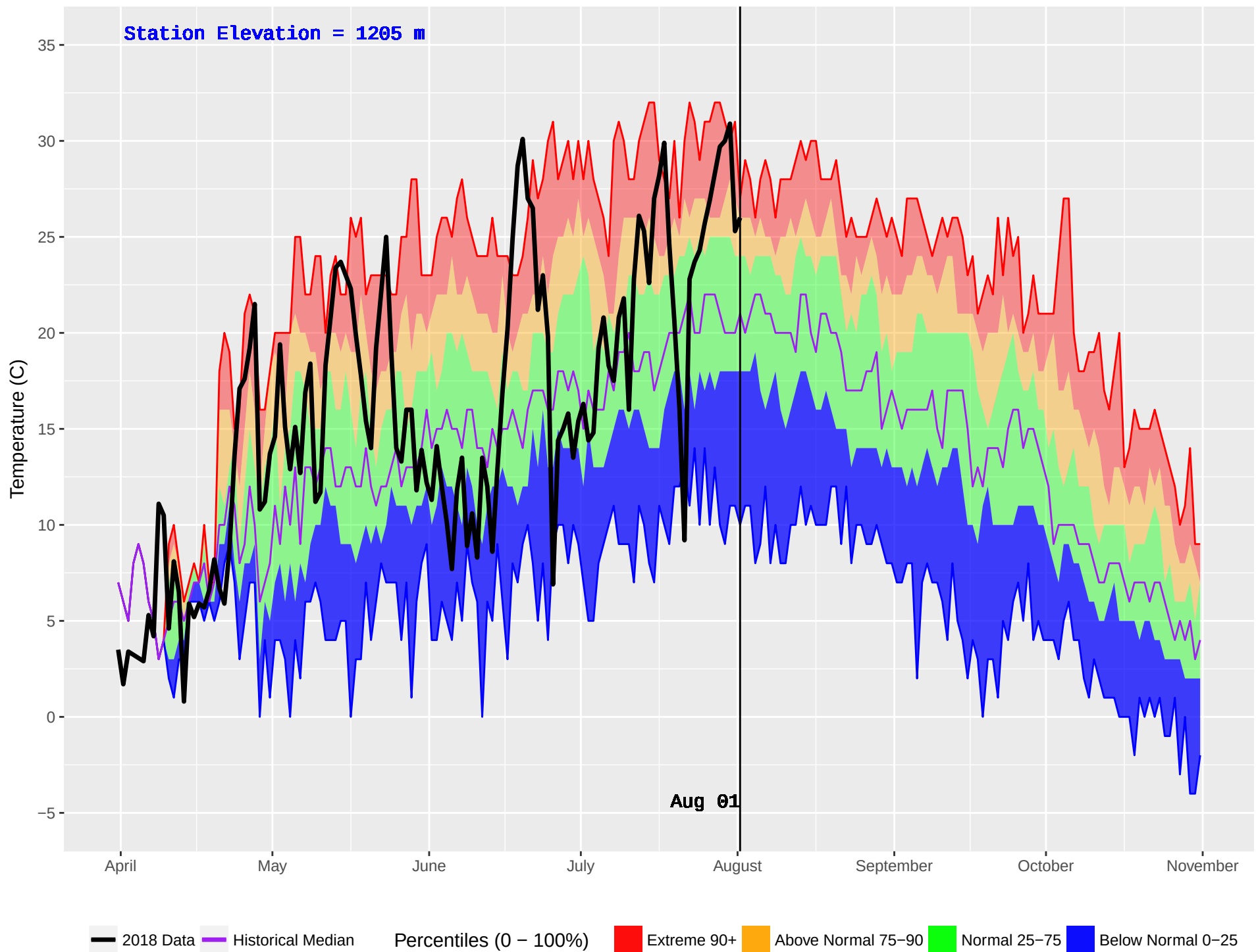
GWYNETH LAKE (309) : Historical (1986–2016) and Current (2018) Daily Temperature
