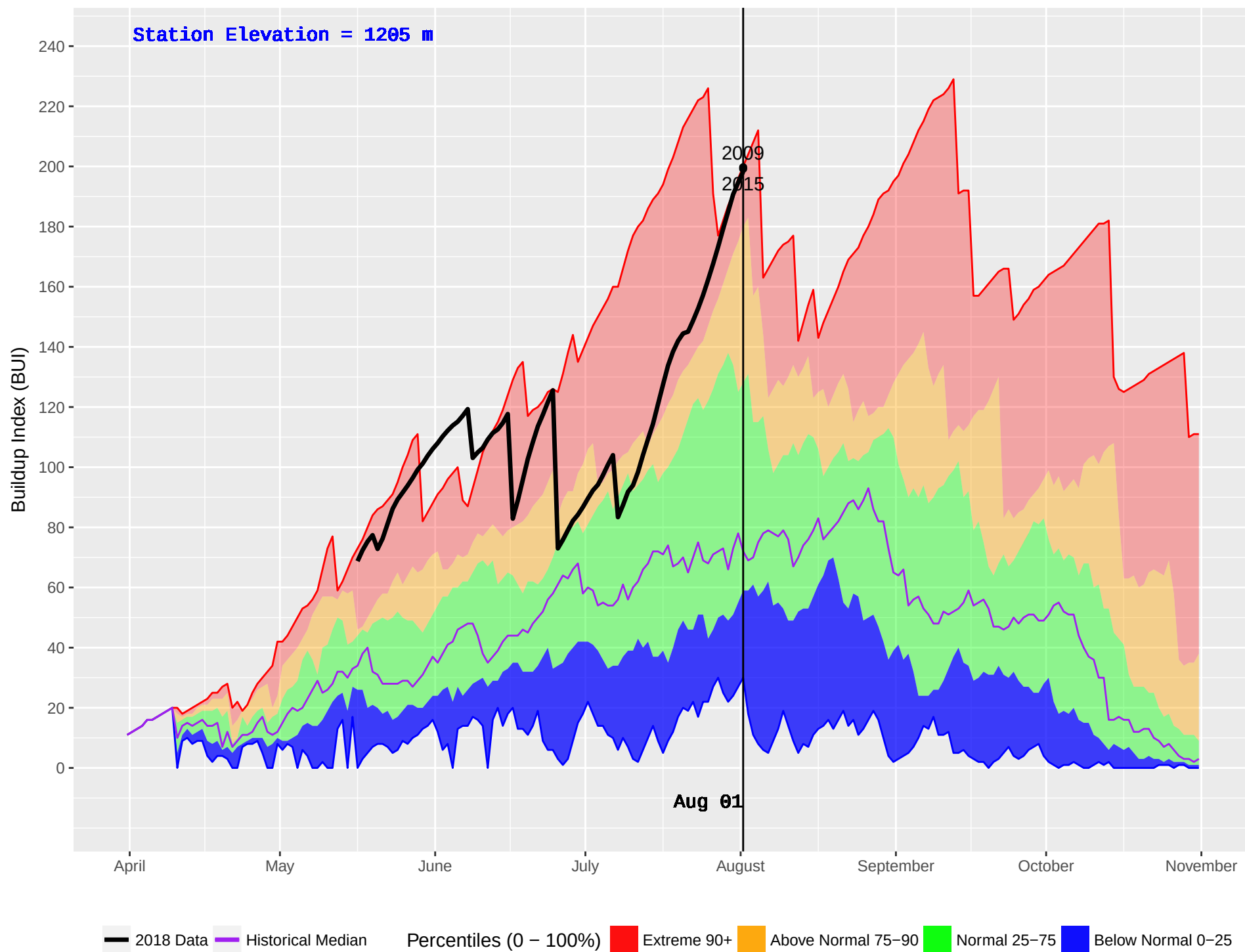
GWYNETH LAKE (309) : Historical (1986–2016) and Current (2018) Daily Buildup Index (BUI)
