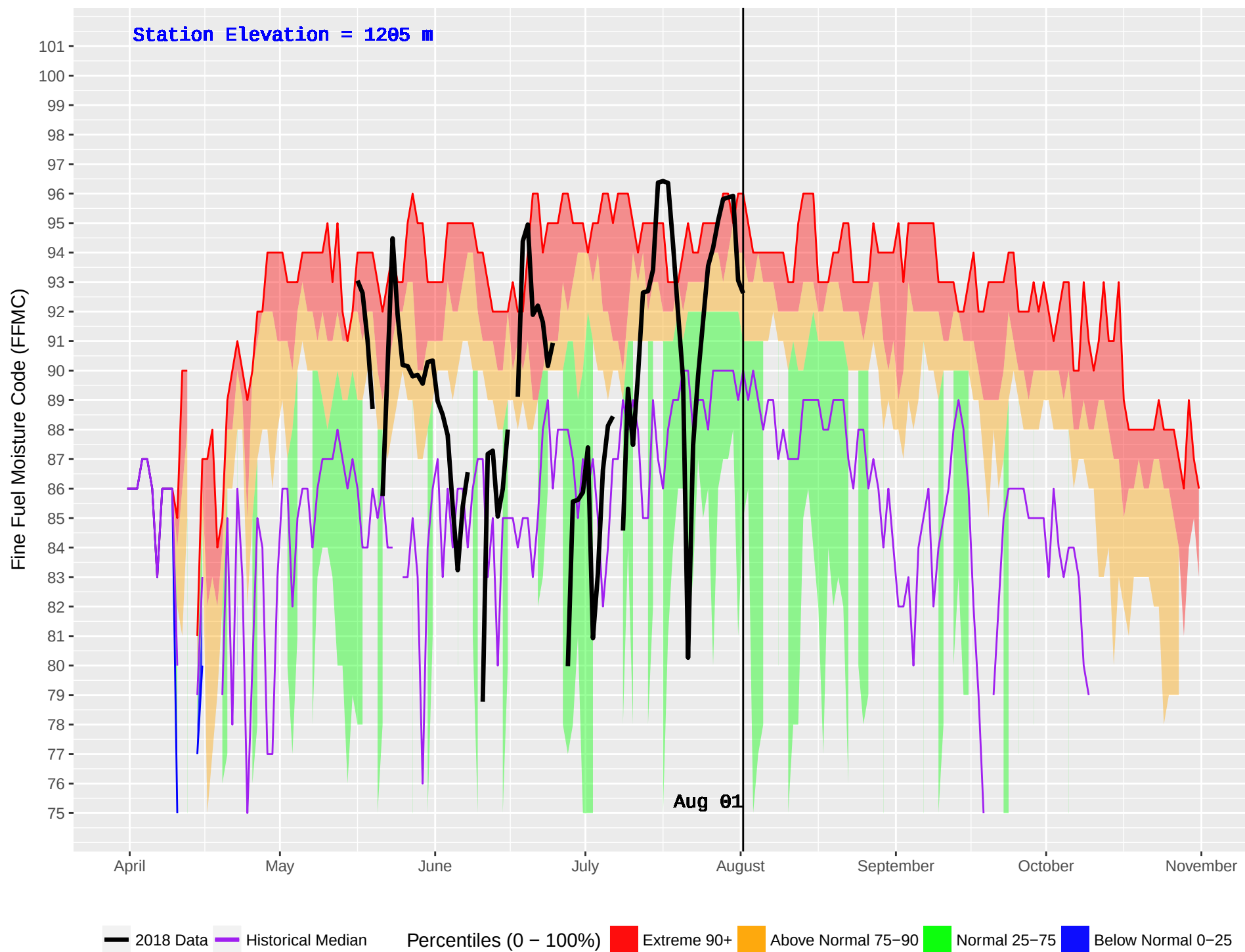
GWYNETH LAKE (309) : Historical (1986–2016) and Current (2018) Daily Fine Fuel Moisture Code (FFMC)
