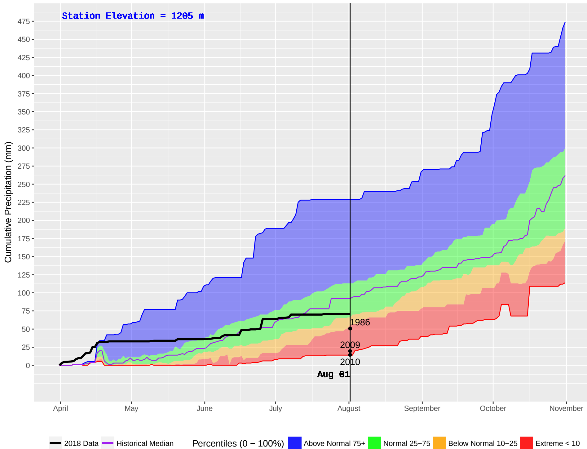
GWYNETH LAKE (309) : Historical (1986–2016) and Current (2018) Daily Cumulative Precipitation
